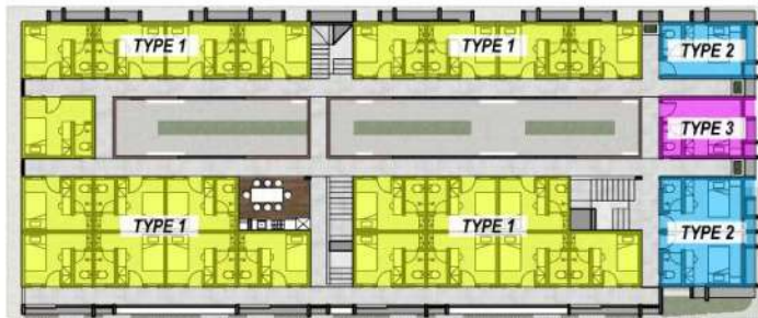
1 DENAH LANTAI 2 - Skala: 1: 300
